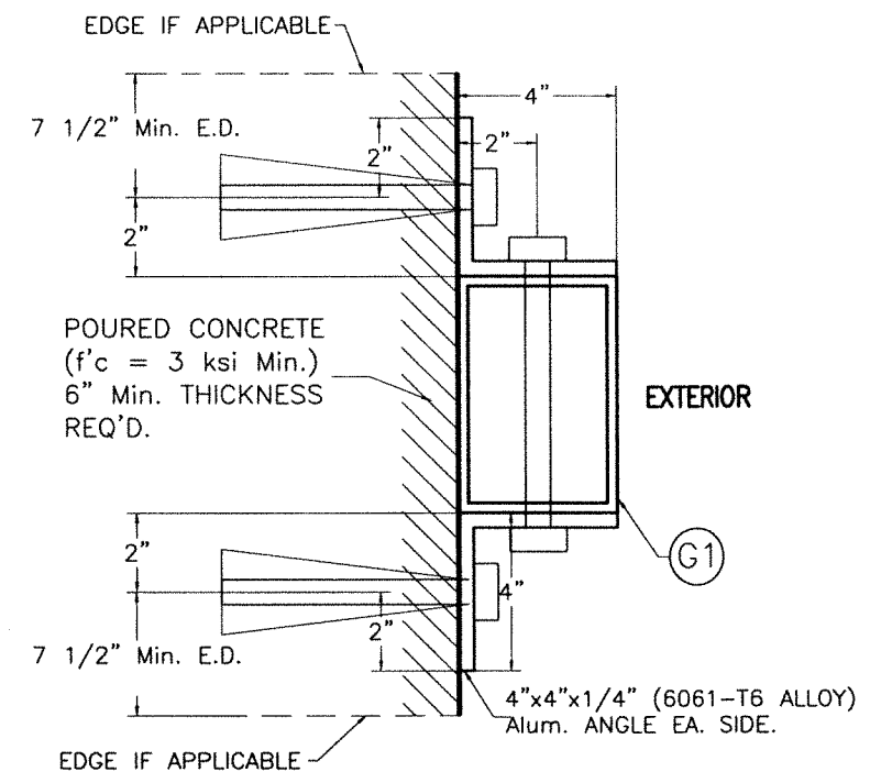
ALTERNATIVE SECTION X2-X2 W/ (G1)* (END & INTERIOR MULLIONS) (W/ ORIENTATION # 1) (8"x4")
