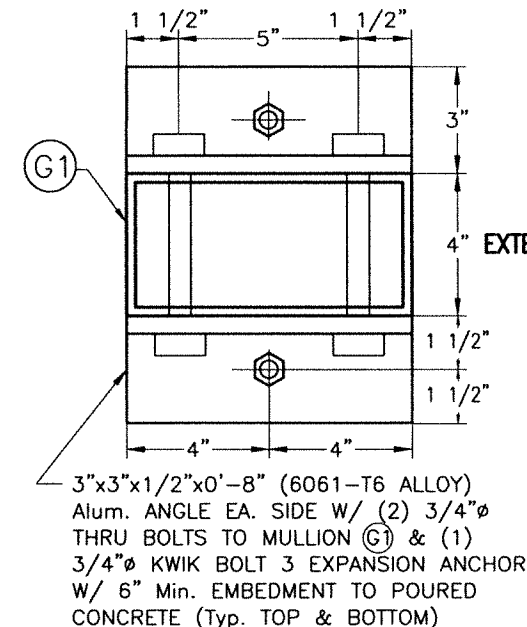
SECTION X1-X1 W/ G * (END & INTERIOR MULLION) (W/ ORIENTATION # 1) (6"x4")
