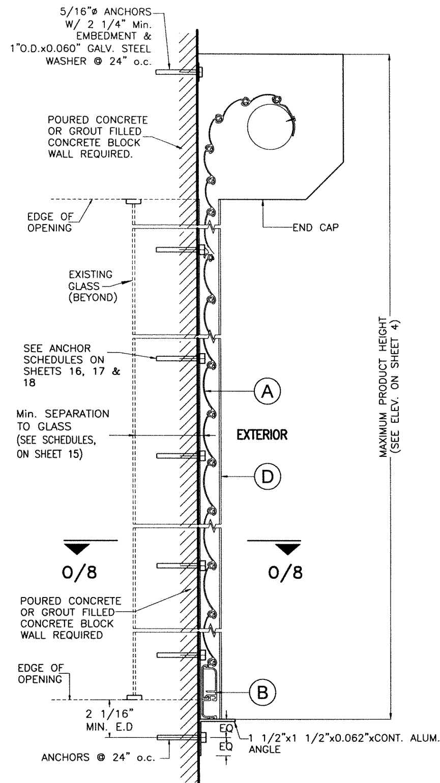
WALL MOUNTING *
