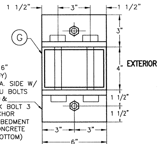
ALTERNATIVE SECTION X1-X1 W/ G * (END & INTERIOR MULLION) (W/ ORIENTATION # 2) (4"x6")
