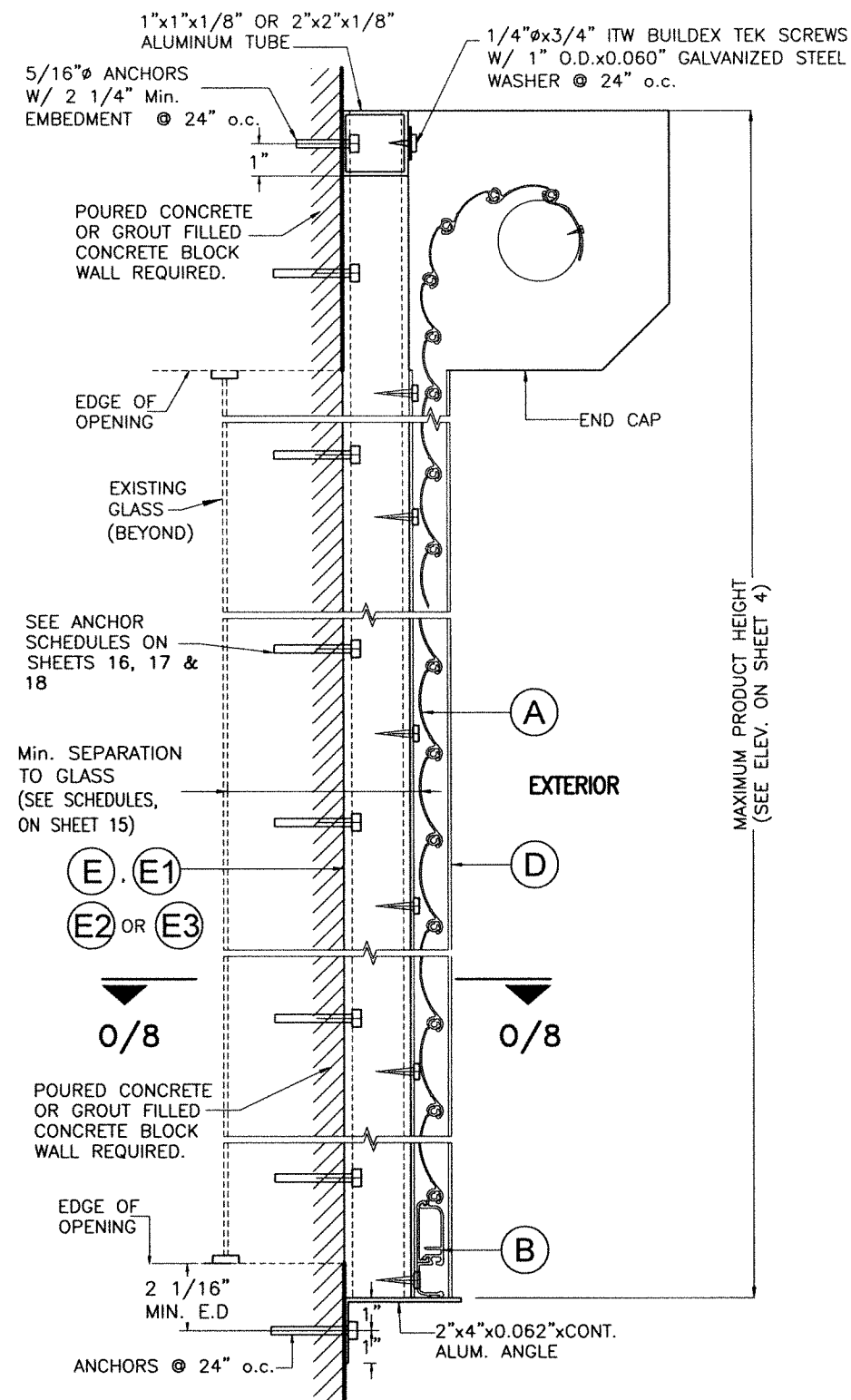
BUILD-OUT MOUNTING *
