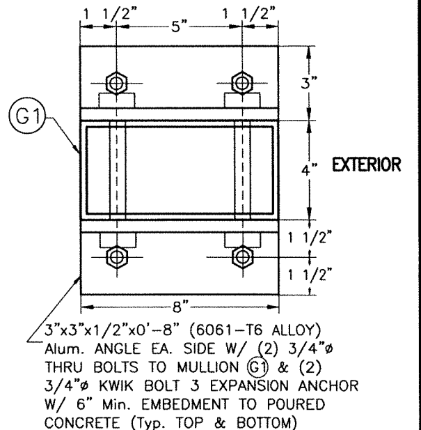
ALTERNATIVE SECTION X1-X1 W/ G * (END & INTERIOR MULLION) (W/ ORIENTATION # 2) (4"x6")
