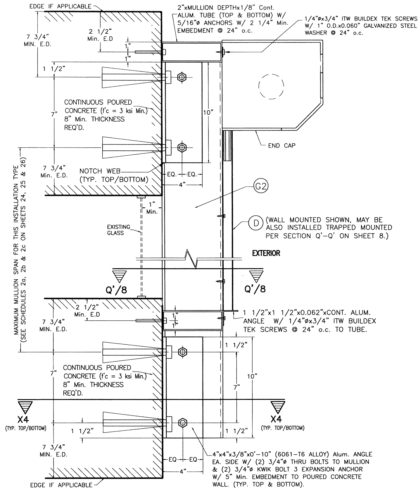
WALL MOUNTING : MULLION G2 POURED CONCRETE WALL SECTION W-4
