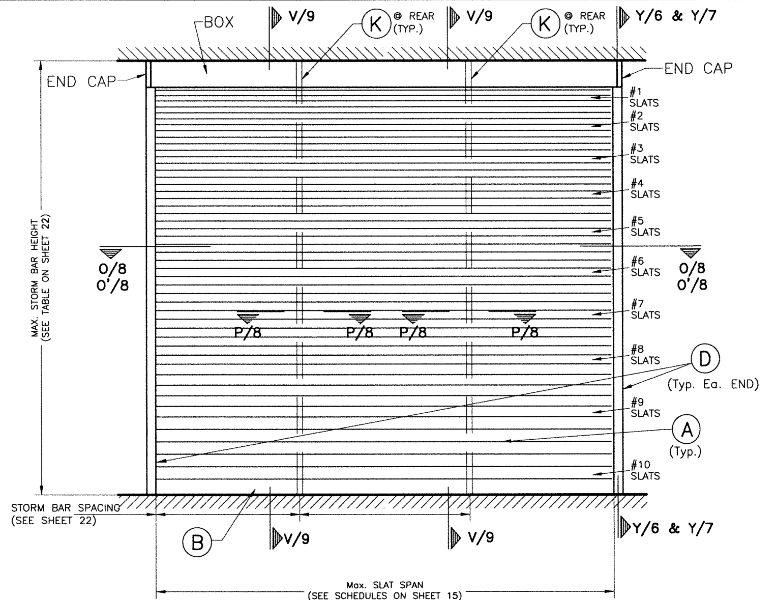
TYPICAL SINGLE UNIT ELEVATION W/ STORM BARS *
