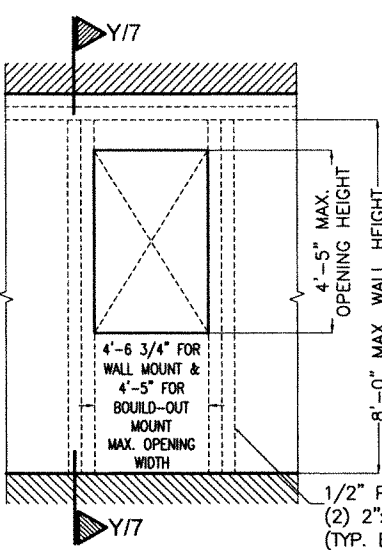
DETAIL 1 (ELEVATION)
