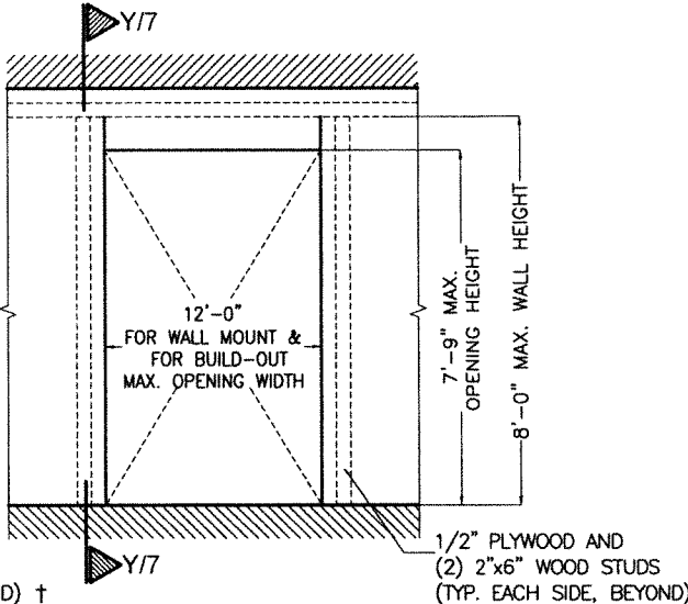
DETAIL 2 (ELEVATION)
